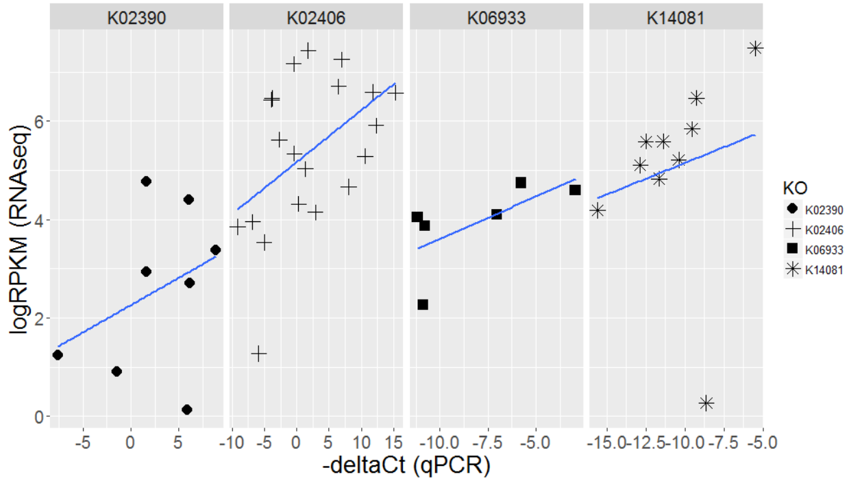
Supplemental Figure S2. Quantitative reverse transcription PCR (qPCR) analysis of select genes for baseline RNA samples from this study. The values represent the logRPKM values from the RNA-Seq result compared to -\Delta Ct values from the qPCR result. Regression lines in blue are presented for each KO. Positive correlations between RNAseq and qPCR were detected for all the tested KOs.
