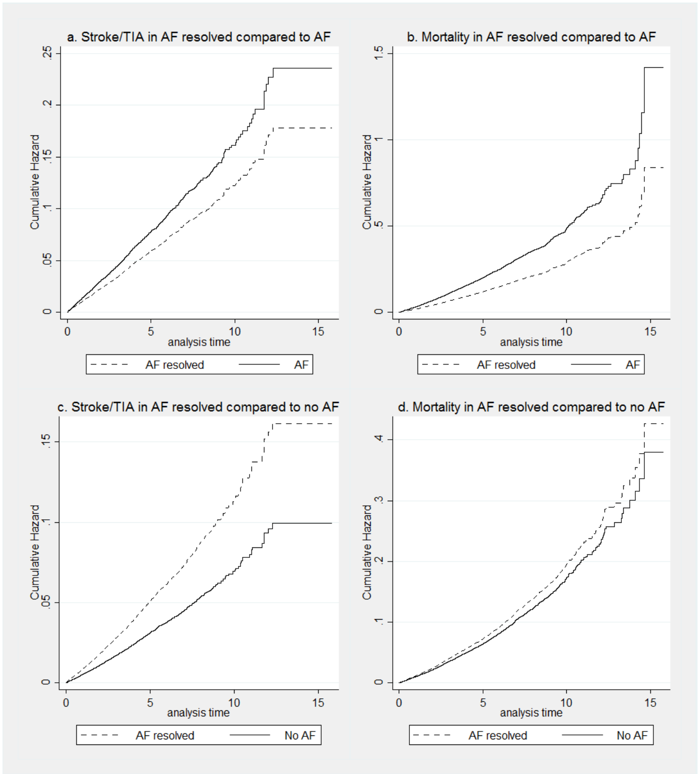
Supplementary Figure 1. Adjusted cumulative hazard estimates for a. stroke/TIA and b. mortality in patients with resolved compared to unresolved AF, and c. stroke/TIA and d. mortality in patients with resolved AF compared to patients without AF.
