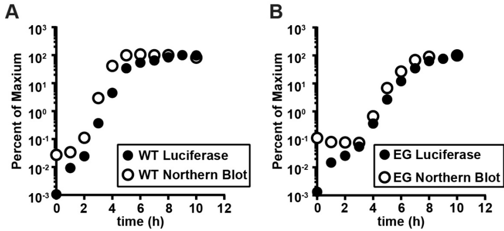
S1 Fig. Comparison of the kinetics of luciferase activity and RNA accumulation by Northern blotting for WT and EG subgenomic replicon. (A,B) Kinetics of RNA replication of subgenomic replicon RNA by WT (panel A) and EG (panel B) as measured by luciferase activity and Northern blotting. Values are represented as percent of the maximum value from each respective assay.
