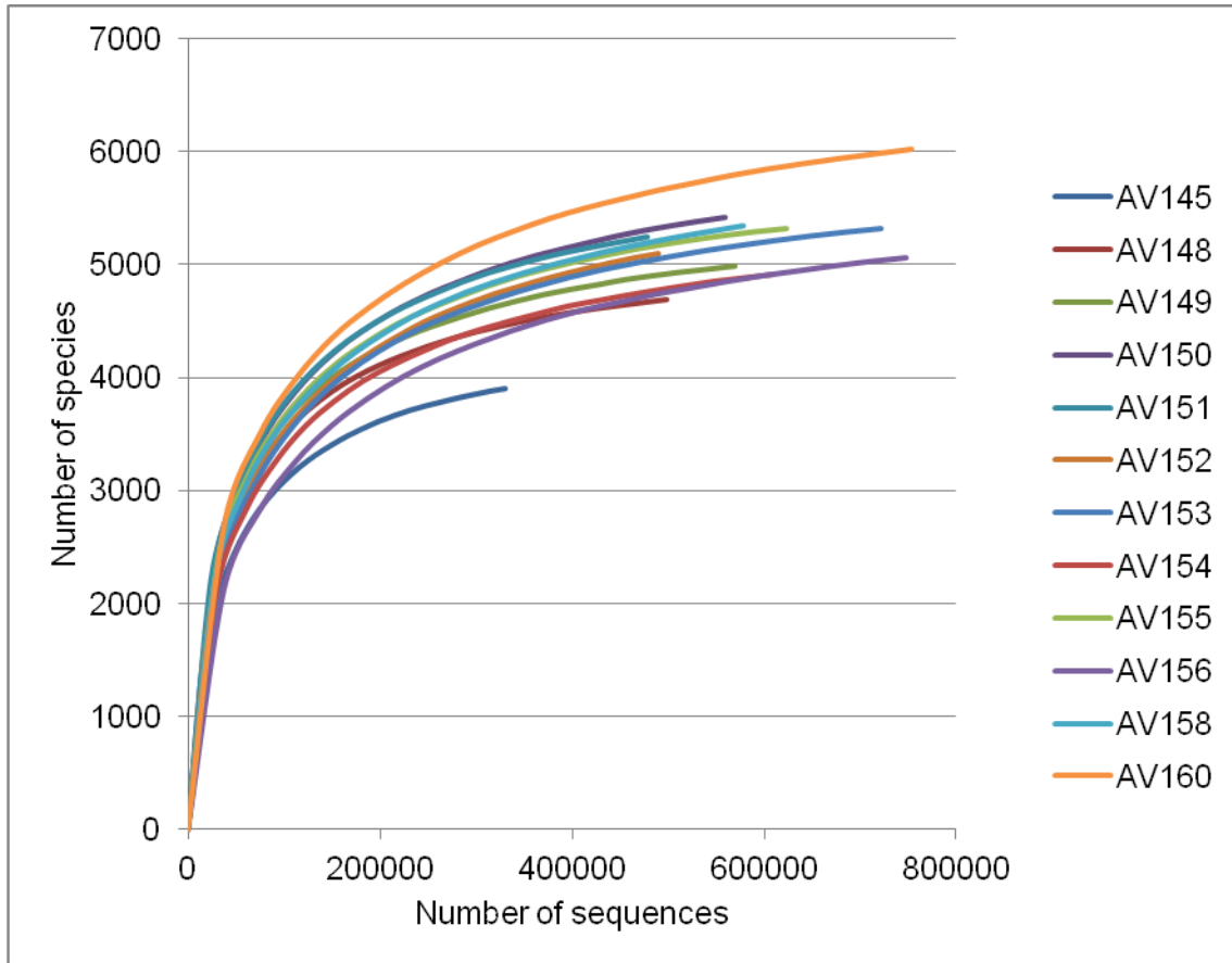
FIGURE S2. Rarefaction curves for mRNA sequences from suppressive (AV145-AV152) and non-suppressive (AV153-AV160) samples assigned at species level on the basis of NCBI taxonomy and lowest common ancestor hierarchy in MEGAN.
