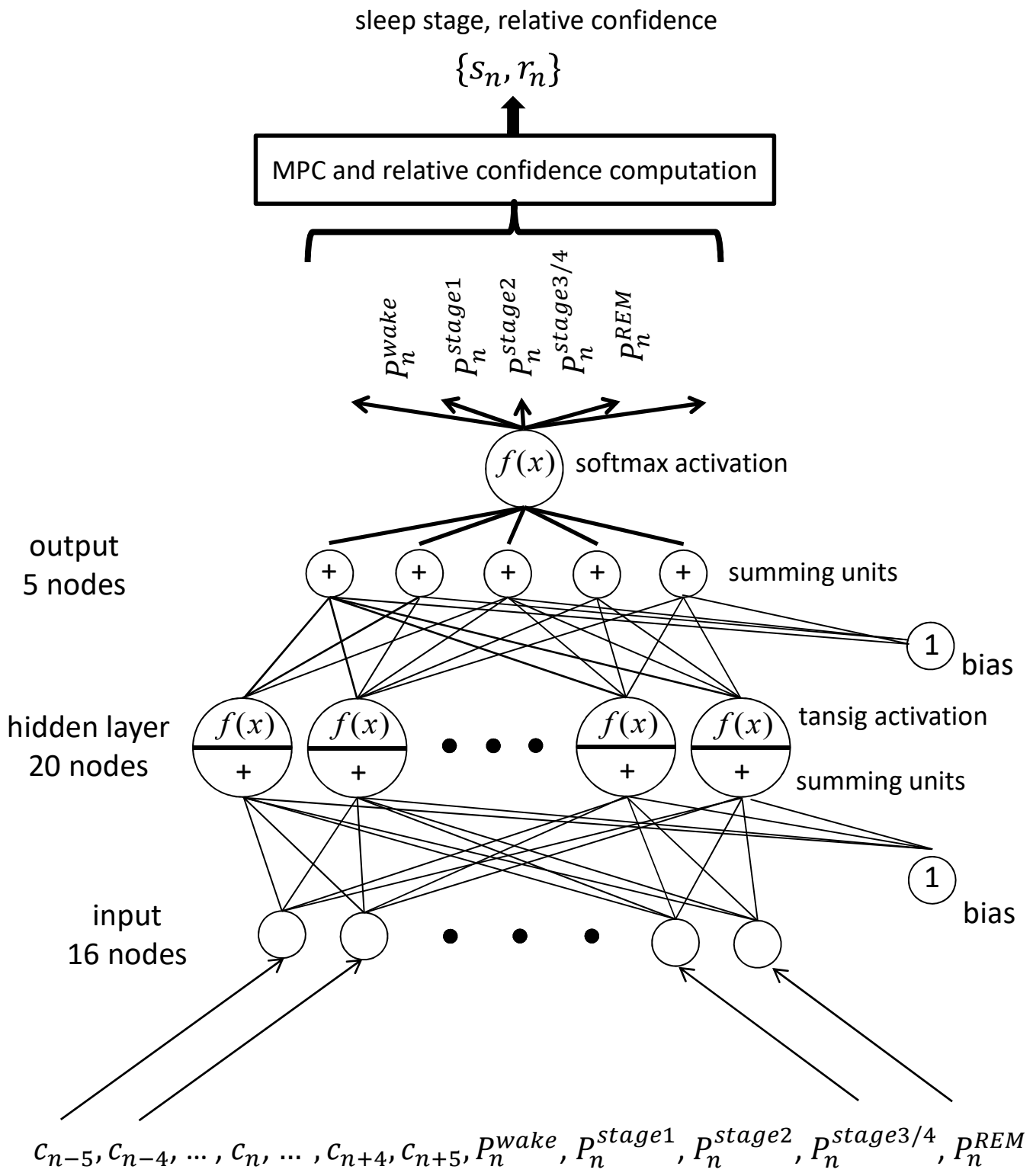
classification block 2
