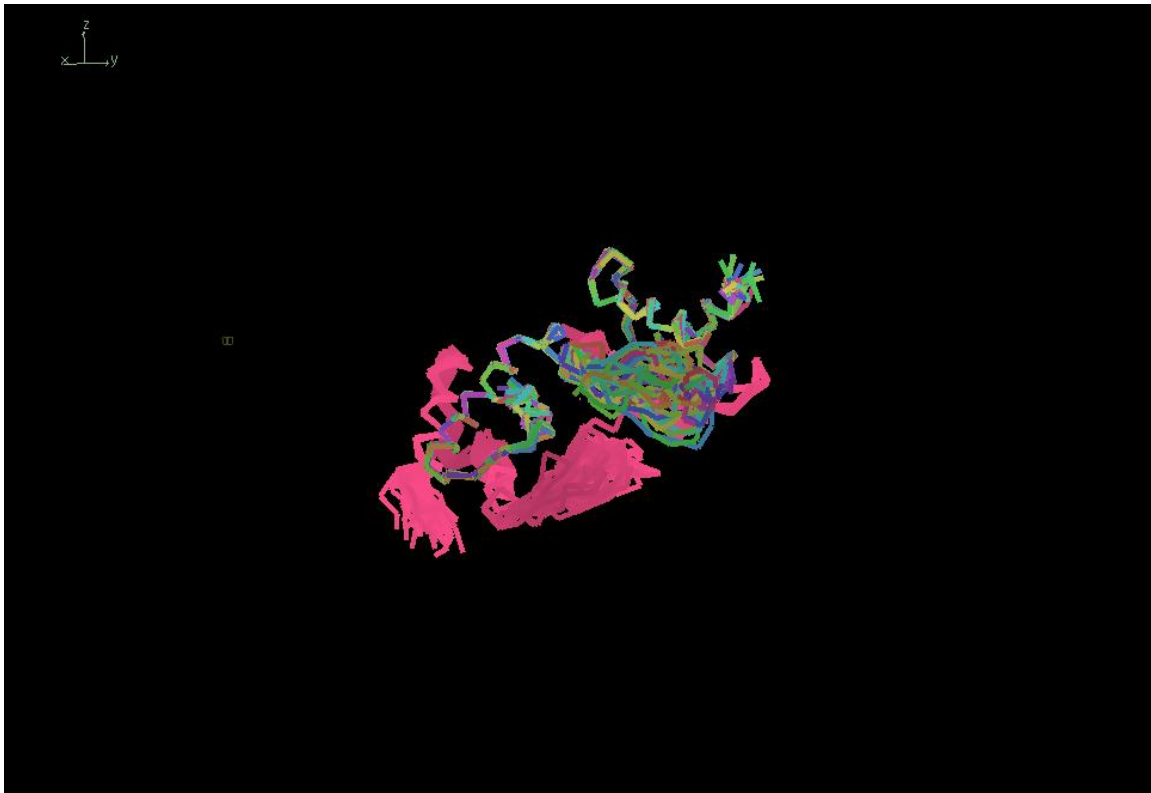
Figure S1 Flexible loops A55-A67; B53-B63 and the termini explore degrees of freedom as a rigid body.
