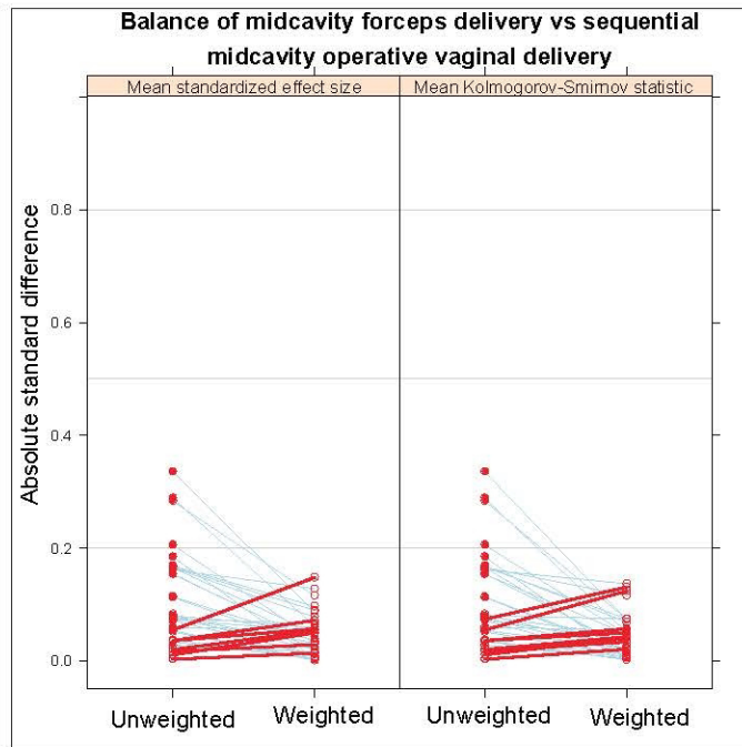
Figure S2. Unweighted and weighted effect size plots for the dystocia cohort. These plots compare the absolute standardized mean differences between the mode of delivery groups on the study covariates, before and after weighting. Absolute standardized mean differences of <0.20 in the weighted groups indicate good balance. A statistically significant absolute standardized difference between the weighted and unweighted values is indicated by the solid circle.
