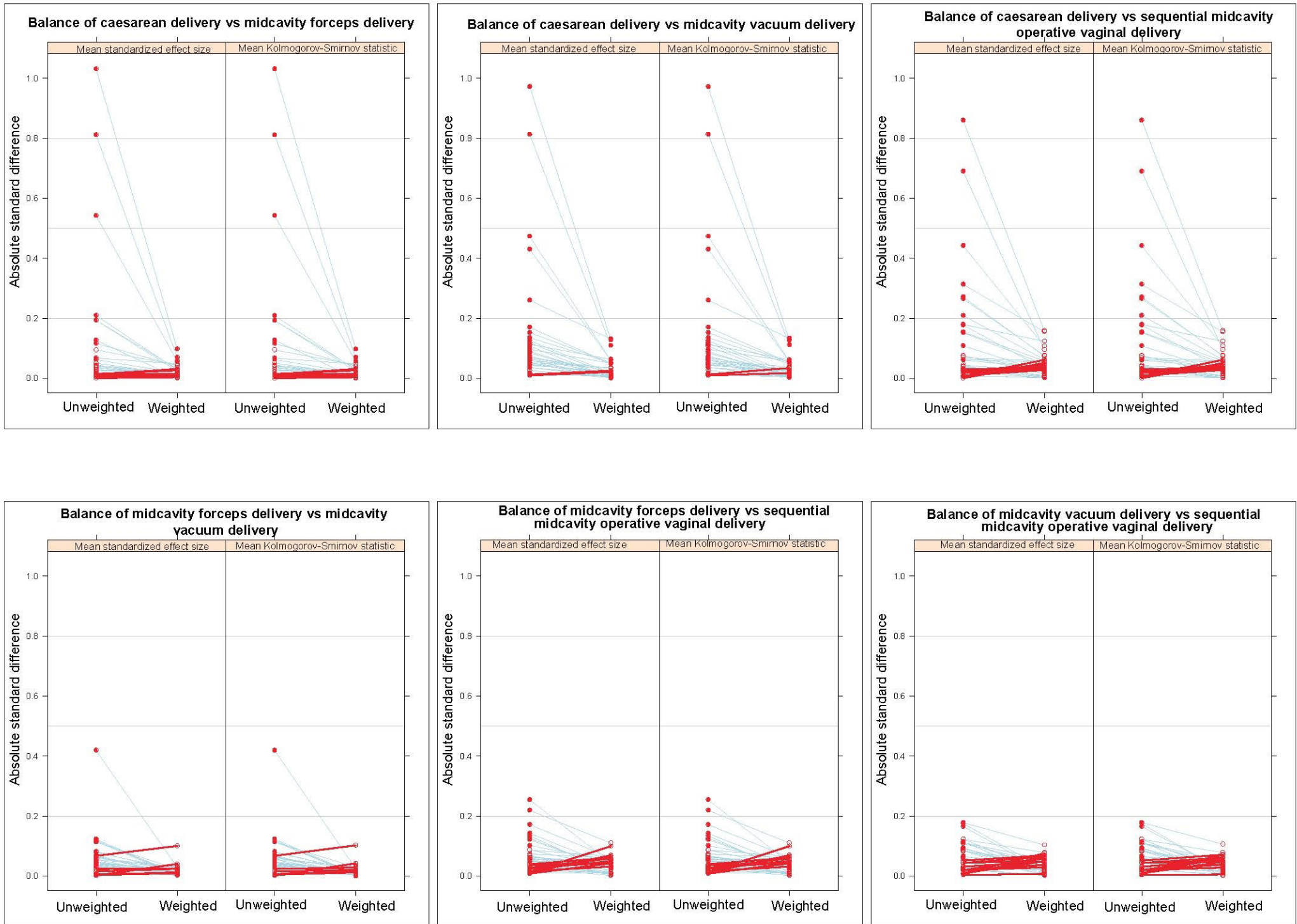
Figure S3. Unweighted and weighted effect size plots for the fetal distress cohort. These plots compare the absolute standardized mean differences between the mode of delivery groups on the study covariates, before and after weighting. Absolute standardized mean differences of <0.20 in the weighted groups indicate good balance. A statistically significant absolute standardized difference between the weighted and unweighted values is indicated by the solid circle.
