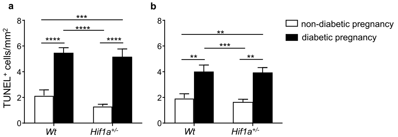
Figure S2. Quantification of TUNEL + apoptotic cells per mm 2 of the RV myocardium (a) and septum (b). The values are mean \pm SEM (n = 4 individuals/3 sections/group). Two-way ANOVA indicating a significant effect of diabetes (RV: P < 0.0001; septum: P < 0.0001) followed by post hoc Tukey's multiple-comparison test, **P < 0.01, ***P < 0.001, **** P < 0.0001.
