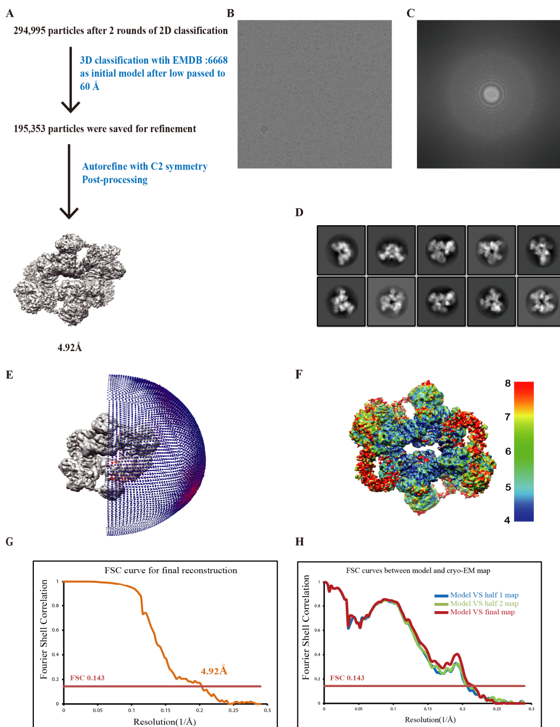
Figure S4 Cryo-EM structure determination of mTORC2. (A) Flow-chart of cryo-EM data processing. (B, C) Representative raw micrograph of cryo-EM mTORC2 (B) and its Fourier transforms (C) . (D) Representative 2D class average of cryo-EM mTORC2
