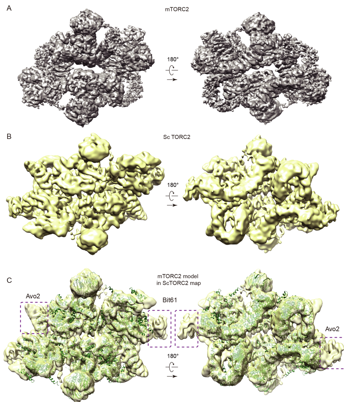
Figure S7 Comparison of the EM maps of mTORC2 and scTORC2. (A, B) Two different views of the EM maps of human mTORC2 at 4.9 Å (A) and scTORC2 at 7.9 Å (B) resolution, respectively. (C) Fitting of the human mTORC2 model into the scTORC2 EM map. Extra densities corresponding to Avo2 and Bit61, the two non-essential components of scTORC2, are indicated.
