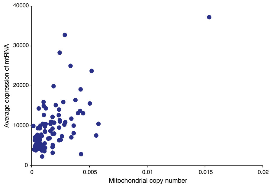
SUPPLEMENTARY FIG. S2. The correlation between mitochondrial copy number and average expression of mtRNA. 100 TCGA thyroid cancer whole-genome sequencing samples were used. A strong correlation between mitochondrial copy number and average expression of mtRNA were observed (Spearman's rank correlation coefficient; r^2=0.583 ).
