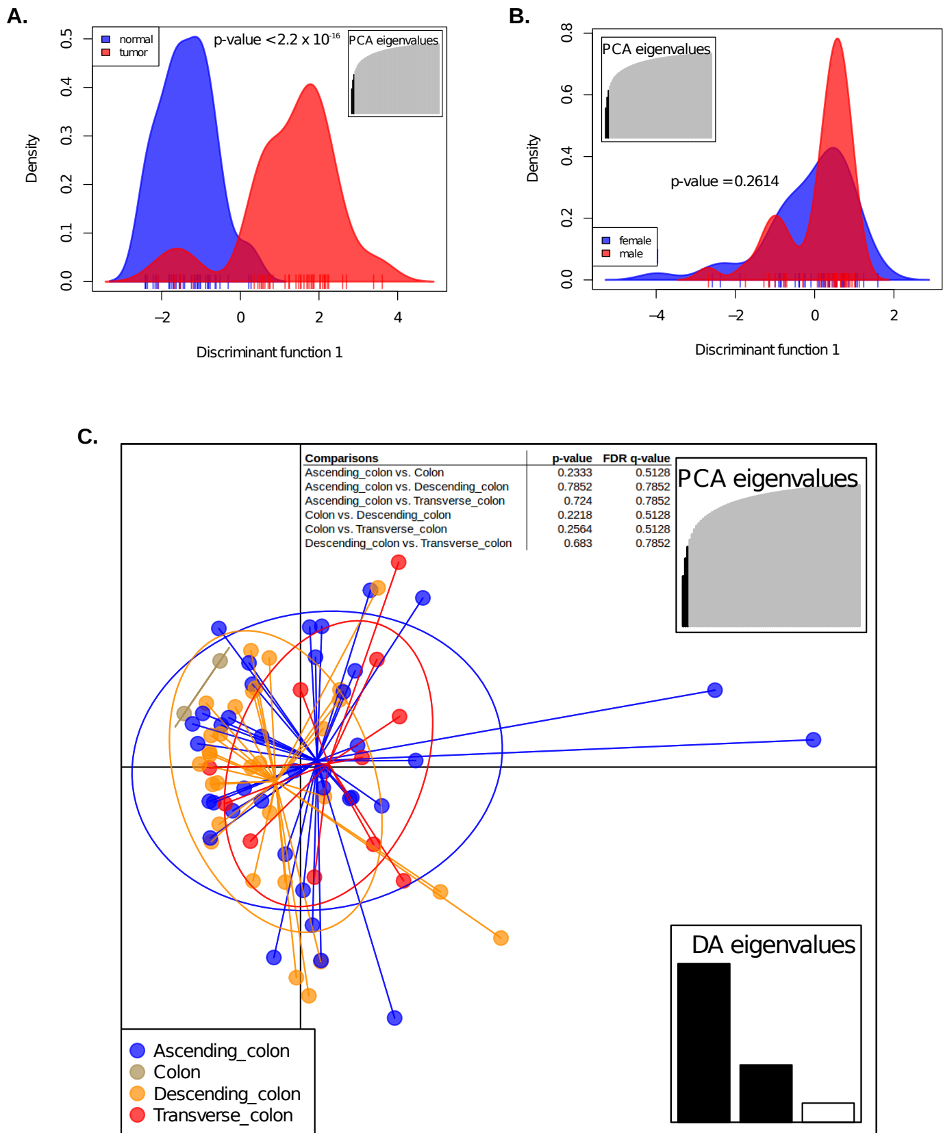
Supplementary Fig. 4. Discriminant analysis of principal components (DAPC) using the first 3 principle components. a. Case status show a clear separation between the tumor and normal groups. b. Genders and c. Tumor location do not affect the does not appear to significantly impact the miRNA expression. Statistical significances are tested using two-sample Kolmogorov-Smirnov test, multiple comparisons are adjusted using false discovery rate (FDR) method.
