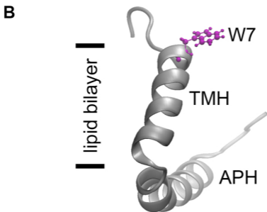
Figure S1: The TMH of TatA begins at Trp-7 (Ref 6) and therefore is very short. (A) Kyte & Doolittle hydropathy plot of TatA (1-60) , (B) NMR structure (PDB 2MN7)
