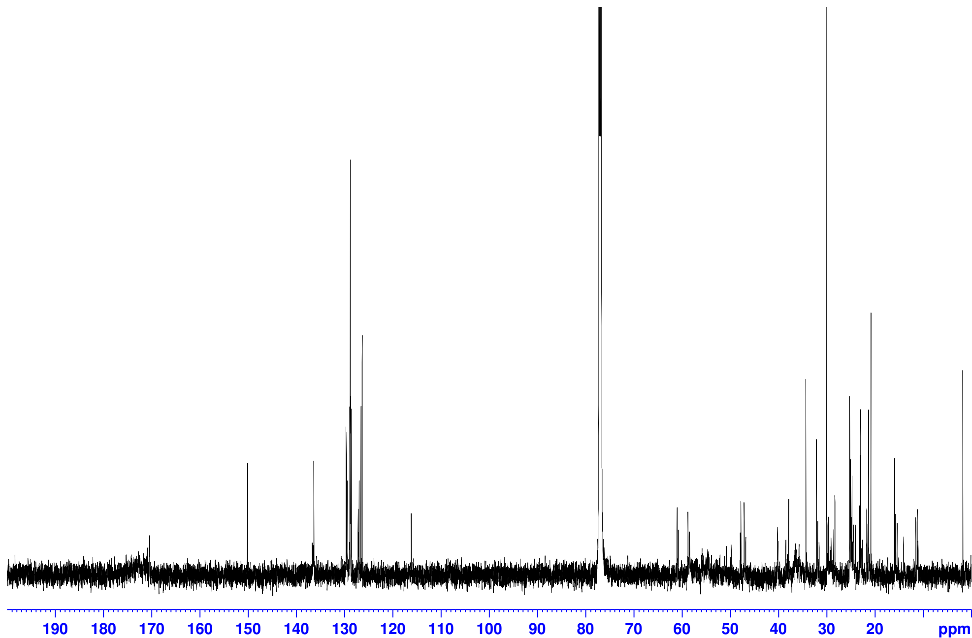
Figure S2. ^{13}\text{C} NMR spectrum of [1-9-N \alpha C]-OLIPPFLLI (19).
