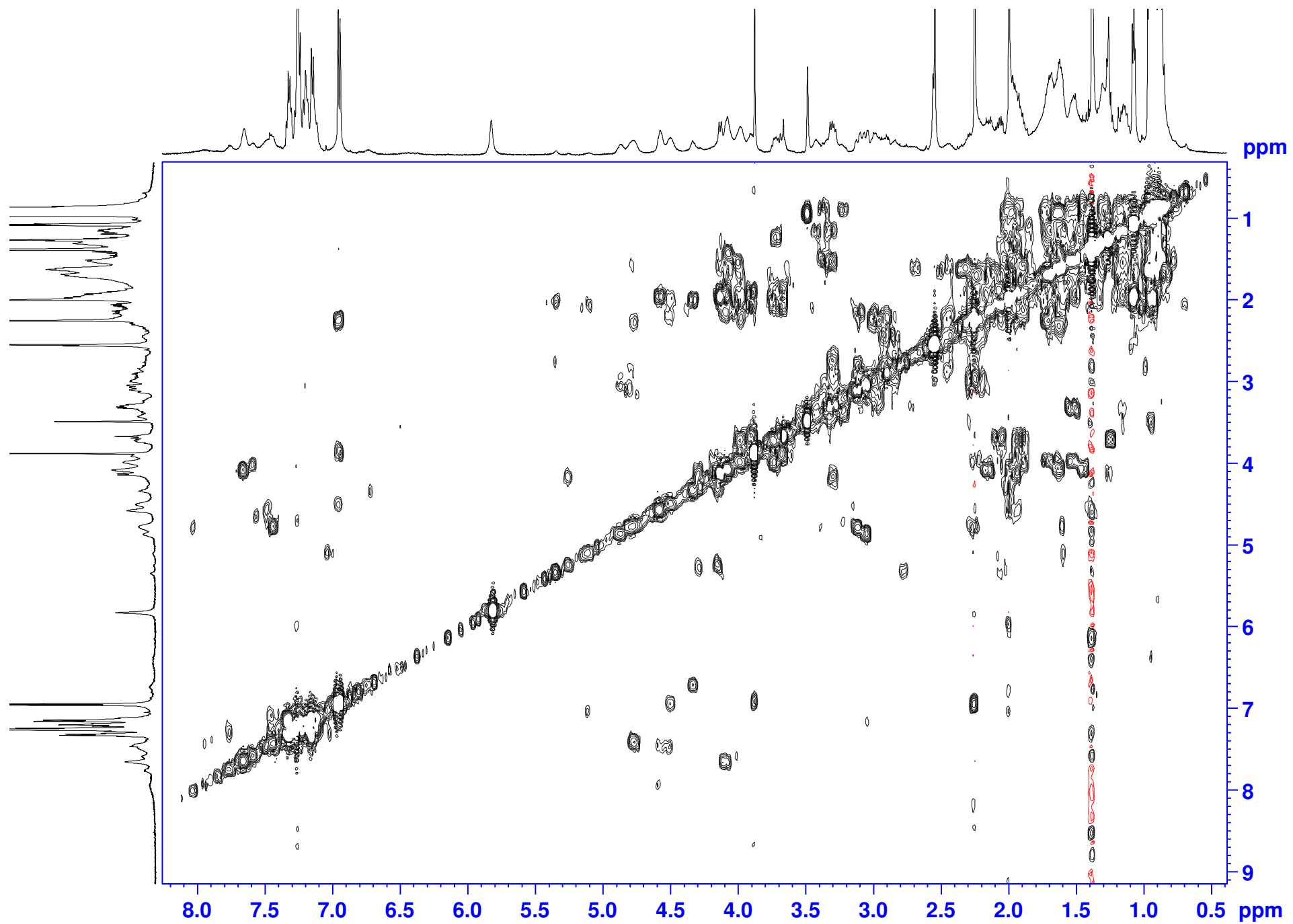
Figure S3. ^1\text{H} - ^1\text{H} COSY spectrum of [1-9-N \alpha C]-OLIPPFLLI (19).
