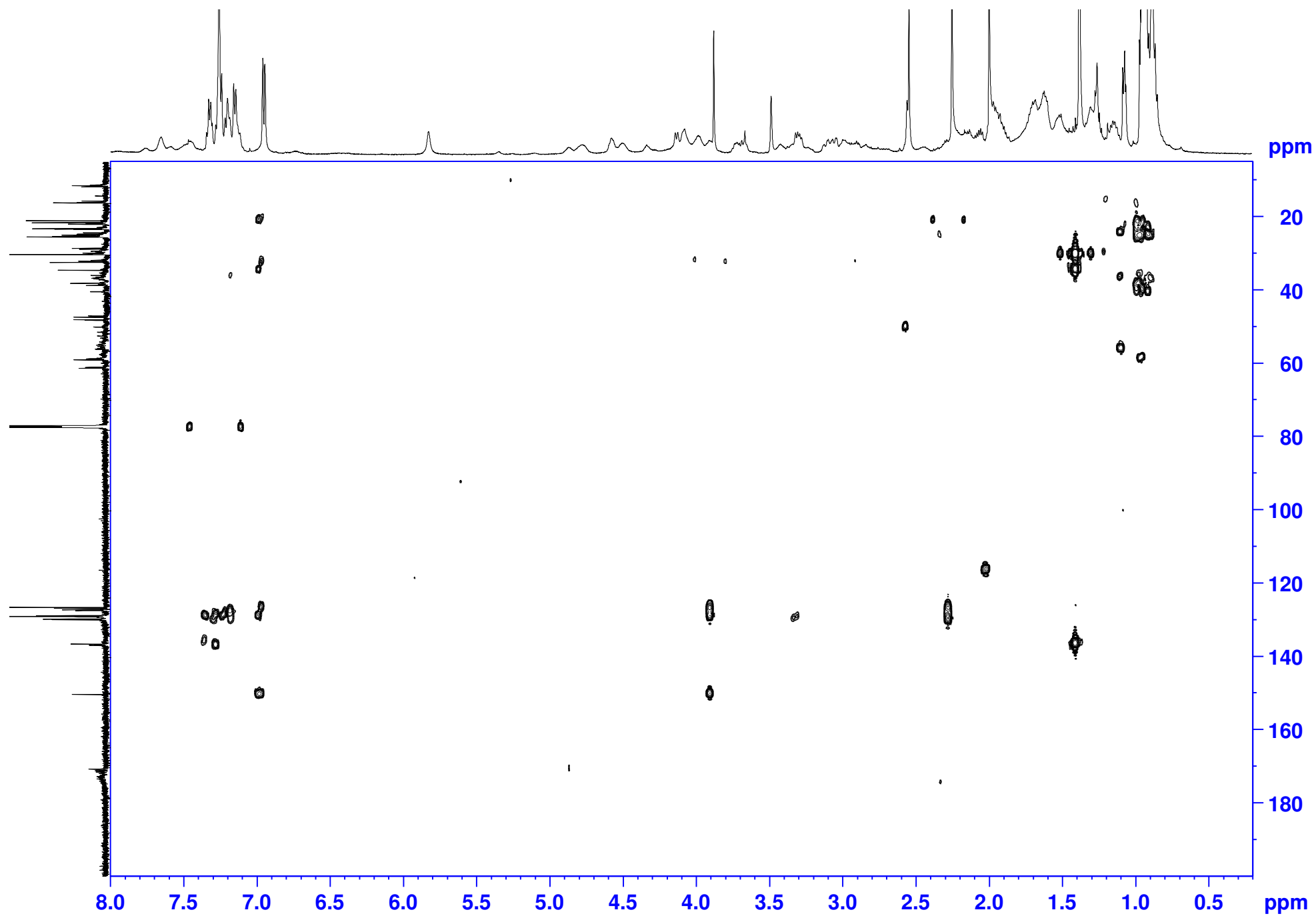
Figure S5. ^1\text{H} - ^{13}\text{C} HMBC spectrum of [1-9-N \alpha C]-OLIPFFLI (19).
