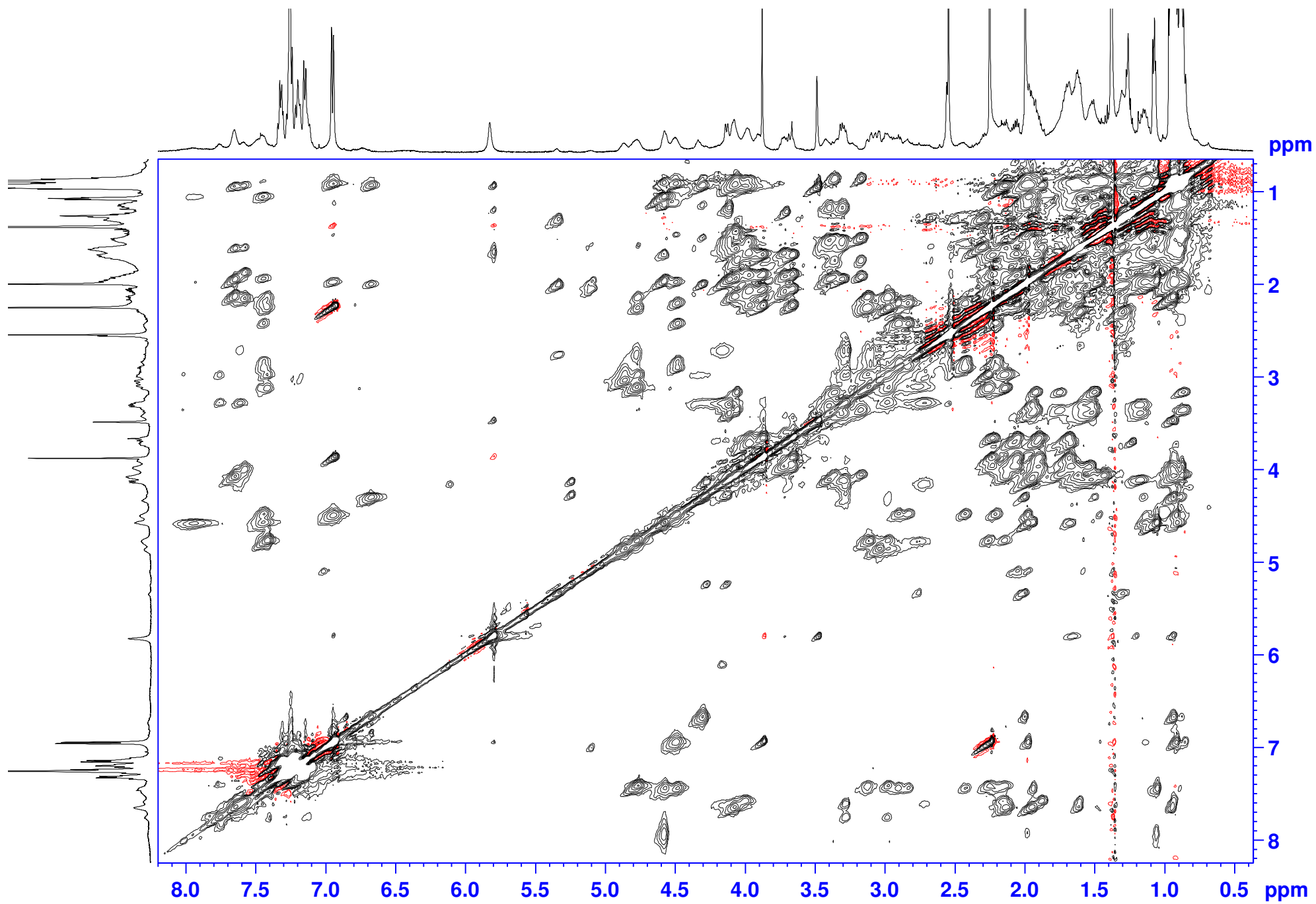
Figure S8. ^1\text{H} - ^1\text{H} TOCSY spectrum of [1-9-NaC]-OLIPFFLI (19).
