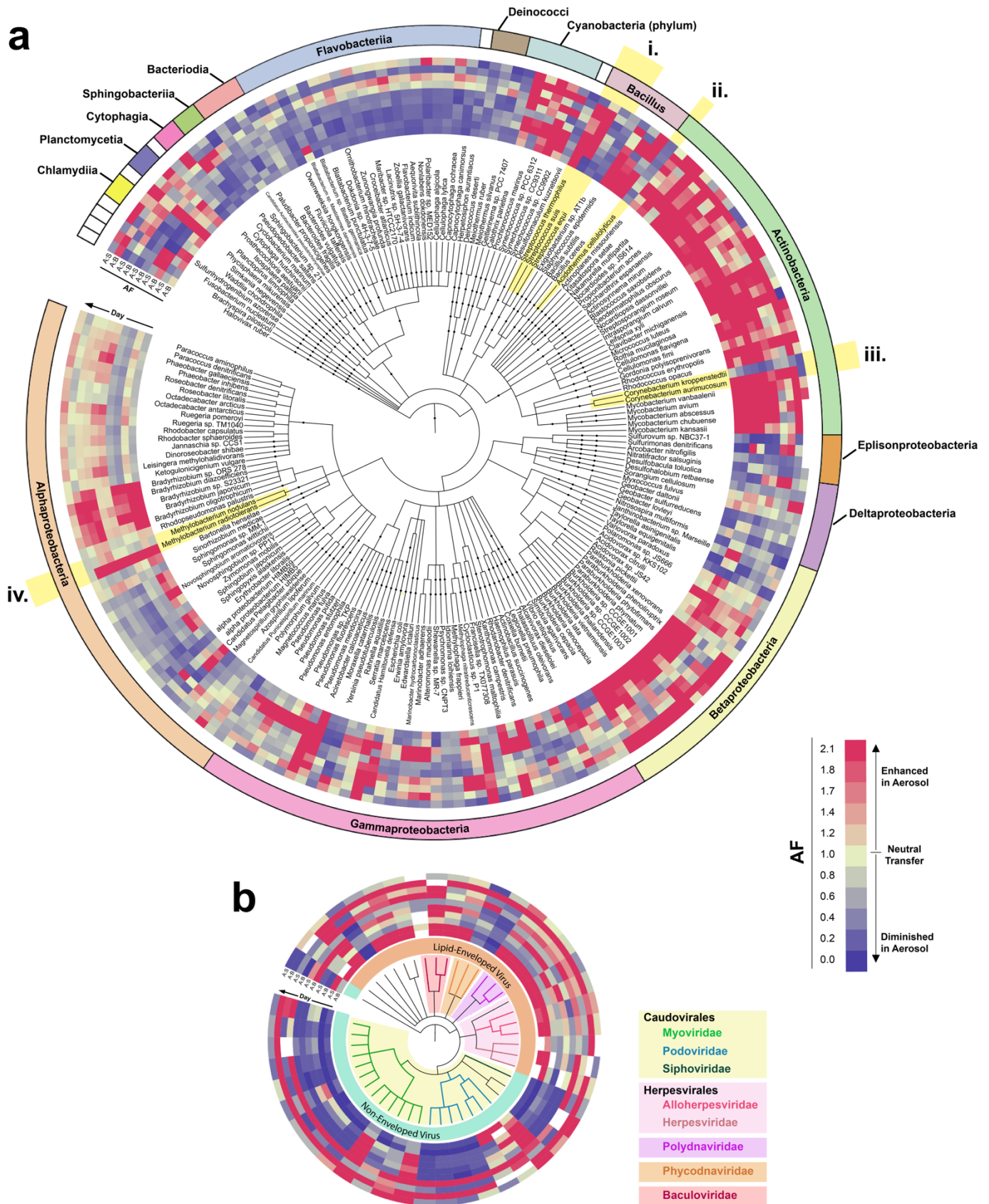
Supplementary Fig. 6 The genetic basis of bacterial and viral aerosolization in the abundance trimmed data set. Genome-based phylogenetic trees based on 197 bacterial genome sequences in a and 46 viral genomes in b . Sequences are derived from read-centric analysis of above 0.1% of the population but not trimmed of genomes with low spatial coverage. The bacteria are a subset of this data that contains 700 bacterial genomes total. The heatmaps display aerosolization factor (AF), A:B and A:S, on different days. AF intensity specified by the legend: Blue = Diminished aerosolization; Yellow = Neutral aerosolization; Red = Enhanced aerosolization. a , Bacteria class is indicated on outer ring to further denote species and aerosolization relationships. Yellow highlights, i–iv indicate closely related species with differing aerosolization patterns. b , Line colors denote viral family and shading indicates order as shown by legend. Additionally, labels on the inner ring specify lipid-enveloped or non-enveloped classifications. Blanks indicate samples below threshold limits.
