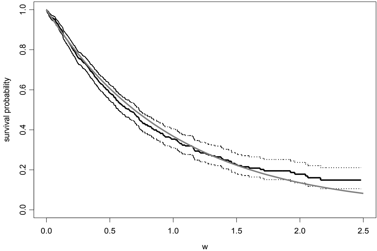
FIGURE S2. Results of cross-validation analysis. This figure shows the standardized times, w_i , (shown collectively as the solid black step curve with 95% confidence intervals as dashed lines) derived from cross-validation and superimposed on the survival function of the standard lognormal LN[0,1] (gray curve).
