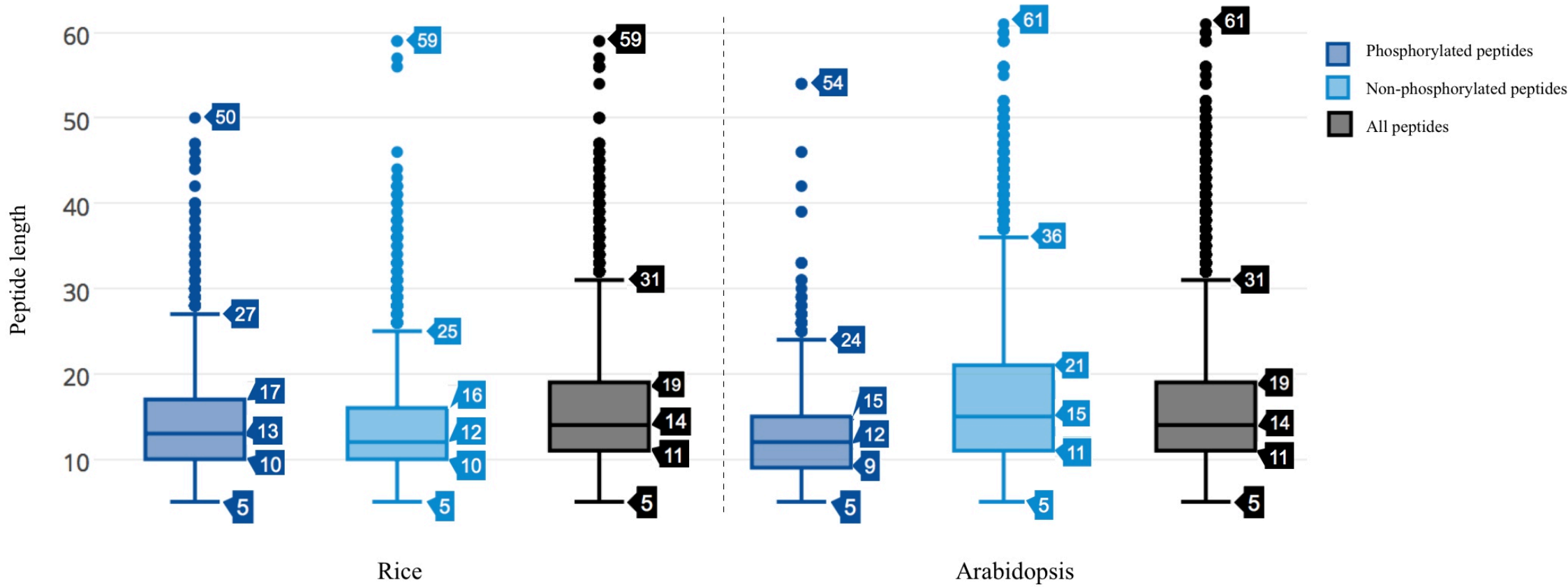
Supplementary Figure 1. The length distribution of phosphorylated, non-phosphorylated and all peptides in rice and Arabidopsis .
