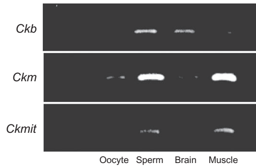
Supplementary Figure S1 The expression of creatine kinase in sperm and oocyte. Because there are three types of brain-type creatine kinase ( Ckb ), muscle-type ( Ckm ) and mitochondria-type ( Ckmit ), the expression of creatine kinase was checked in sperm and oocytes. Oocytes were collected from oviduct at 16 hr after hCG stimulation. Sperm were collected from epididymis and incubated in HTF medium for 1 hr. Total RNA was recovered from oocyte, sperm, brain and muscle, and then used in the RT-PCR study. Brain and muscle were used as positive control.
