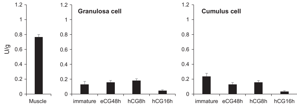
Supplementary Figure S2 The activities of creatine kinase in granulosa cells and cumulus cells. The samples were collected after hormonal treatment. Muscle was used as positive control.
