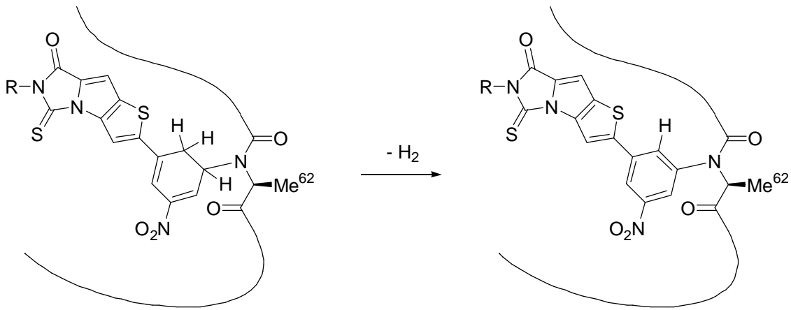
First Neutral IV703/TNFRc1 Adduct
