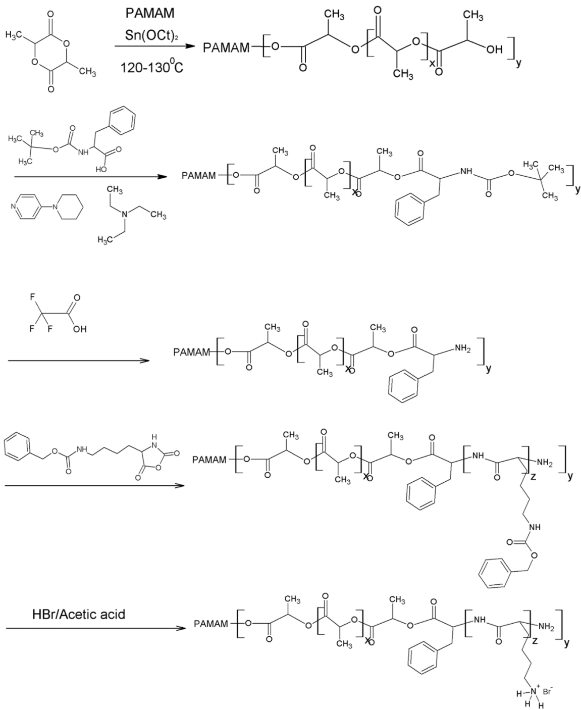
Figure S1. A schematic illustration of the synthesis route of star-shaped block copolymer SS-PLLA-b-PLYS.
