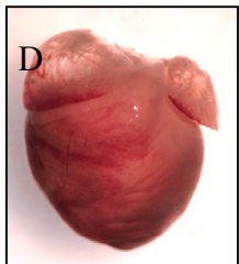
Cre
