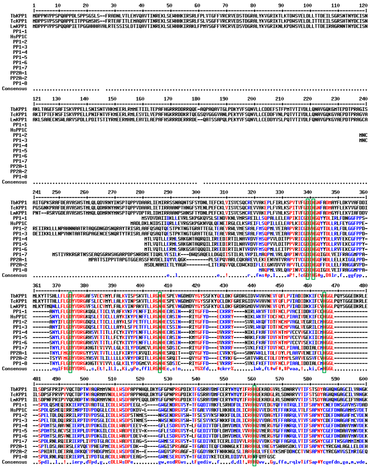
Figure S1. Sequence alignment of the kinetoplast KPP1 homologs, human and T. brucei PP1 homologs, and T. brucei PP2A homologs. The six manganese-coordinating residues are boxed in green boxes. The accession numbers are: TbKPP1: Tb927.5.4380; LmKPP1: LmjF.05.0100; TcKPP1: TcCLB.507601.10; PP1-1: Tb927.11.8090; PP1-2: Tb927.8.7390; PP1-3: Tb927.4.5030; PP1-4: Tb927.4.3640; PP1-5: Tb927.4.3630; PP1-6: Tb927.4.3620; PP1-7: Tb927.4.3560; PP1-8: Tb927.4.3610; PP2A-1: Tb927.3.1240; PP2A-2: Tb927.11.11940; HsPP1C: NP_002701.1.
