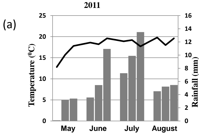
Additional file 3: Figure S3. Climate conditions in rainfed field located in Wohlde (a-b), Walewice (c-d) and Gatersleben (e). Moisture content of soil in the field in Gatersleben location (f). Bars represent rainfall and lines – Temperature (a-e).
