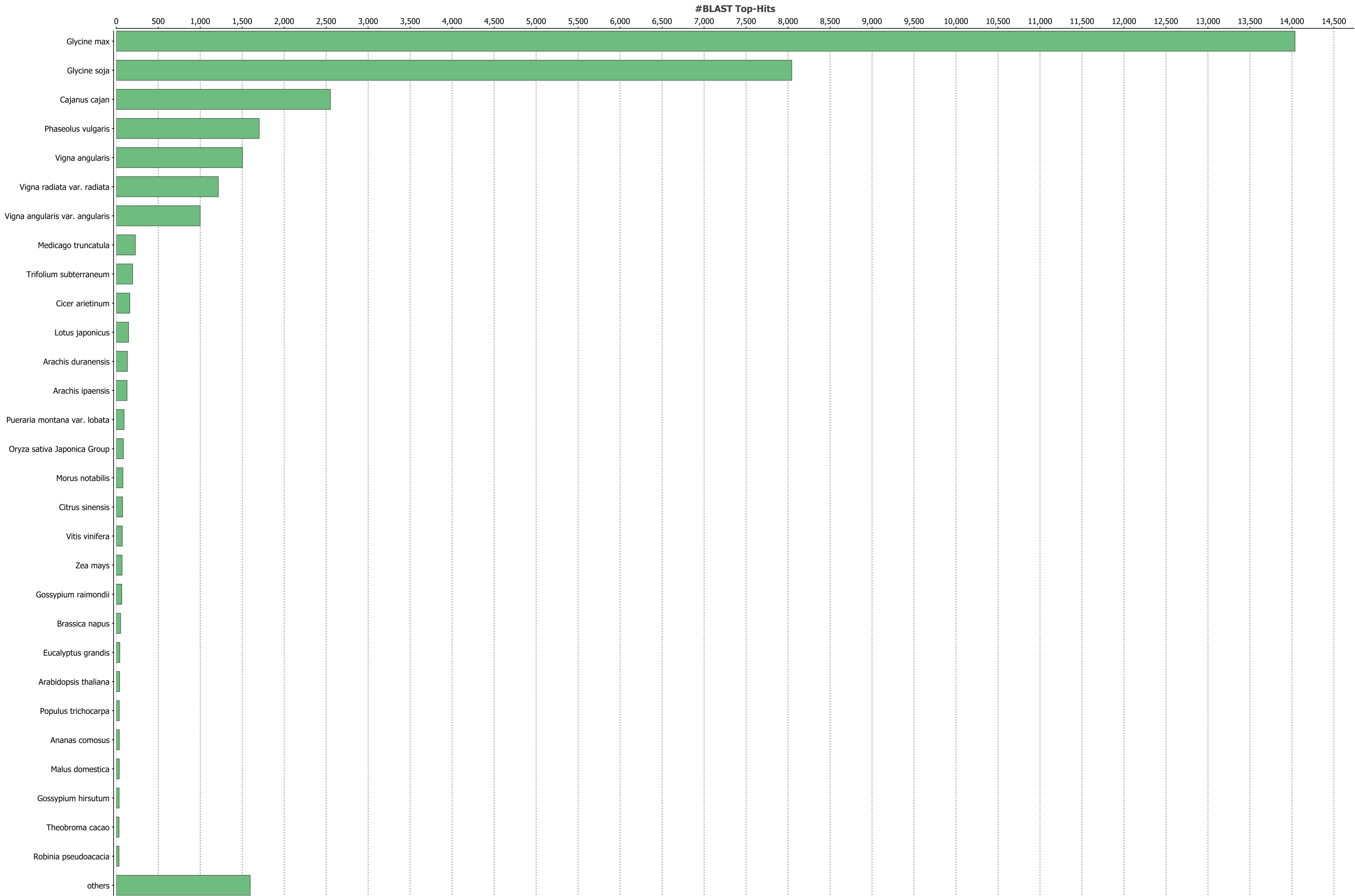
Figure S1: CPP27 Top-Hit Species Distribution
