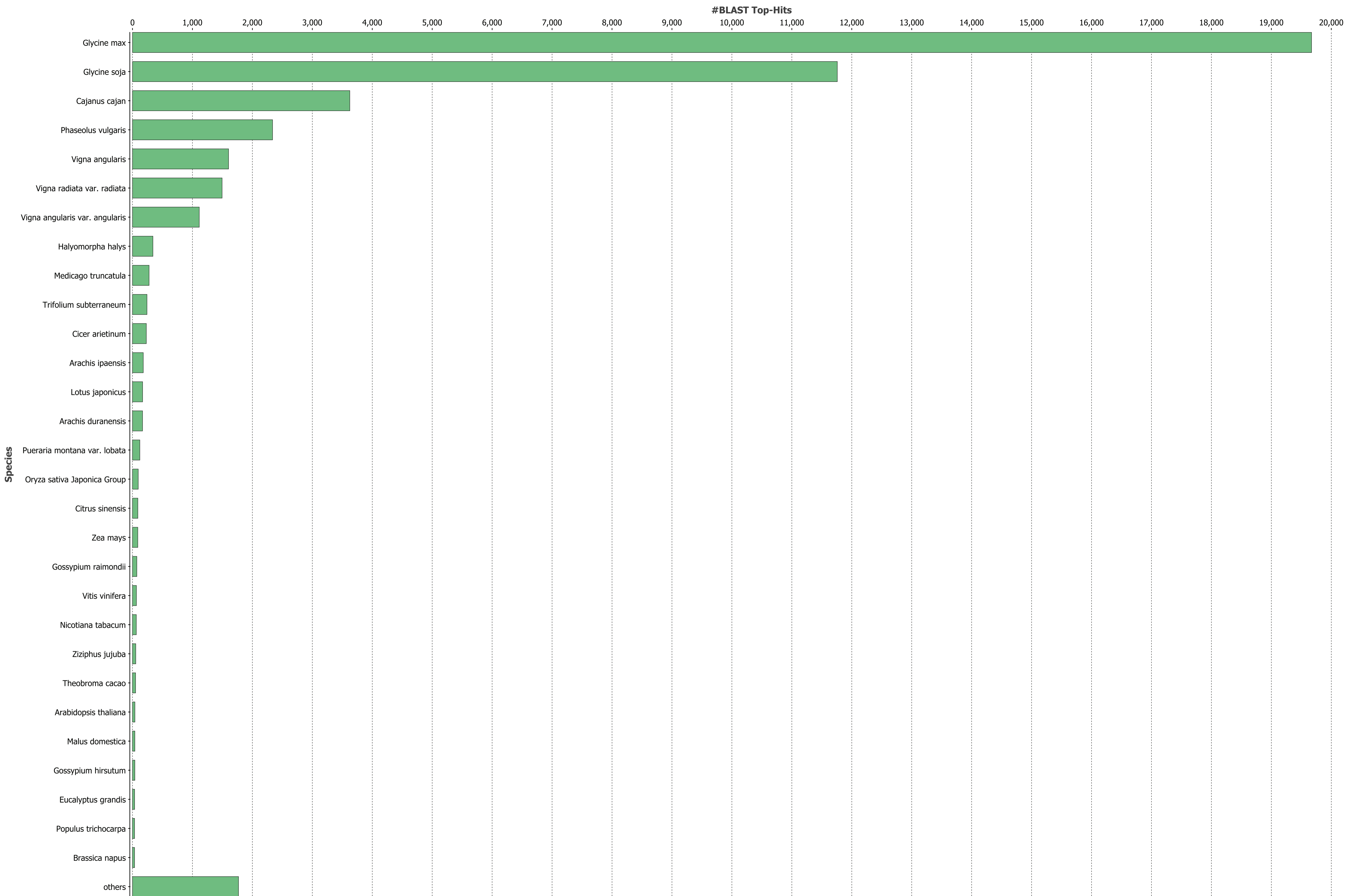
Figure S2: Pmnk6 Top-Hit Species Distribution
