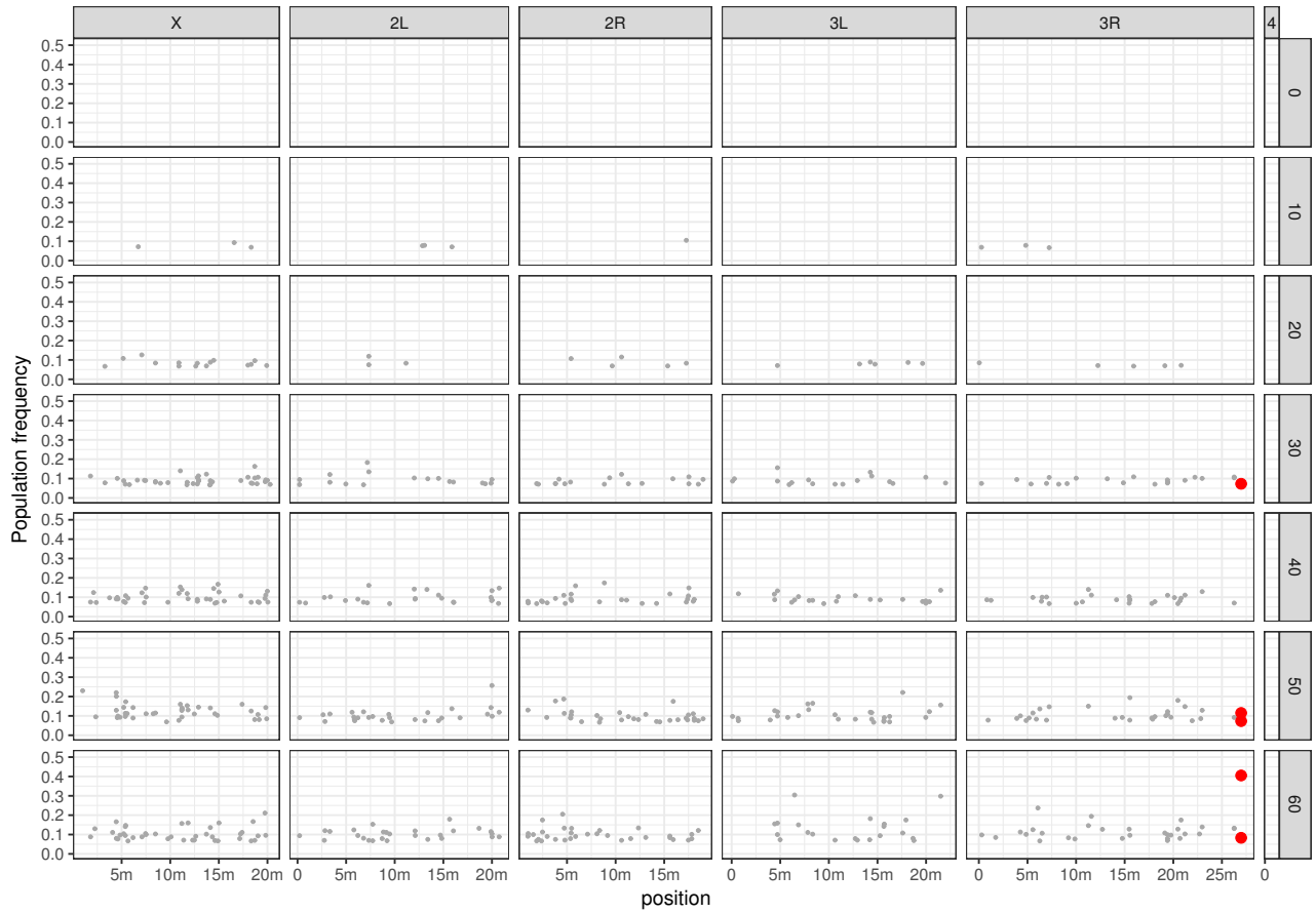
Supplementary Fig. 1: P-element invasion in hot replicate 1. Positions and population frequencies of P-element insertions are shown during the invasion (generations are in the right panel). P-element insertions in piRNA-clusters are shown red. We subsampled the physical coverage to 15 to allow an unbiased comparison of TE abundance between samples. m: million base pairs
