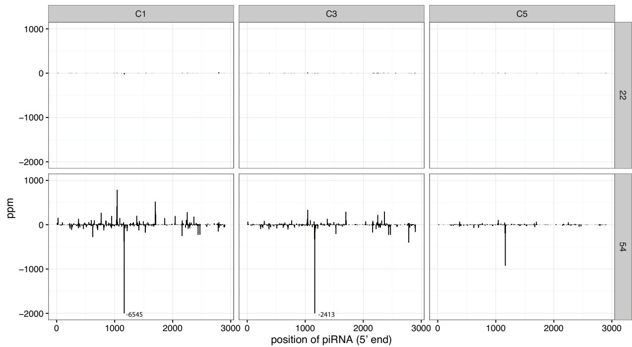
Supplementary Fig. 17: Distribution of piRNAs along the P-element in cold evolved populations. Only the 5' positions of piRNAs are considered and piRNA abundance is normalized to 1 million miRNAs (ppm). Replicates are at the top panel and the generations at the right panel. Sense piRNAs are shown on the positive y-axis and antisense piRNAs on the negative y-axis. Large peaks at positions 1162 were truncated (total size is indicated).
