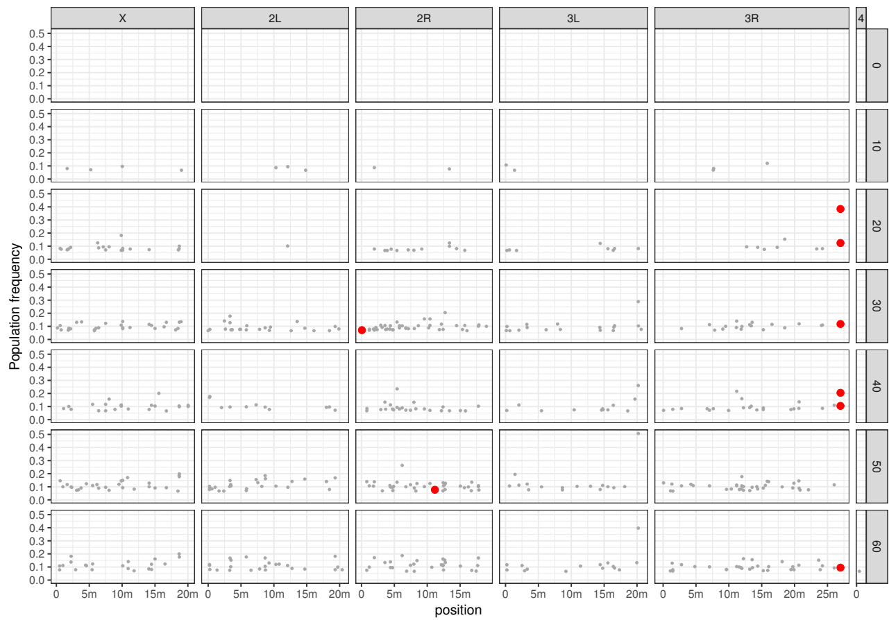
Supplementary Fig. 2: P-element invasion in hot replicate 3. For details see fig. 1.
