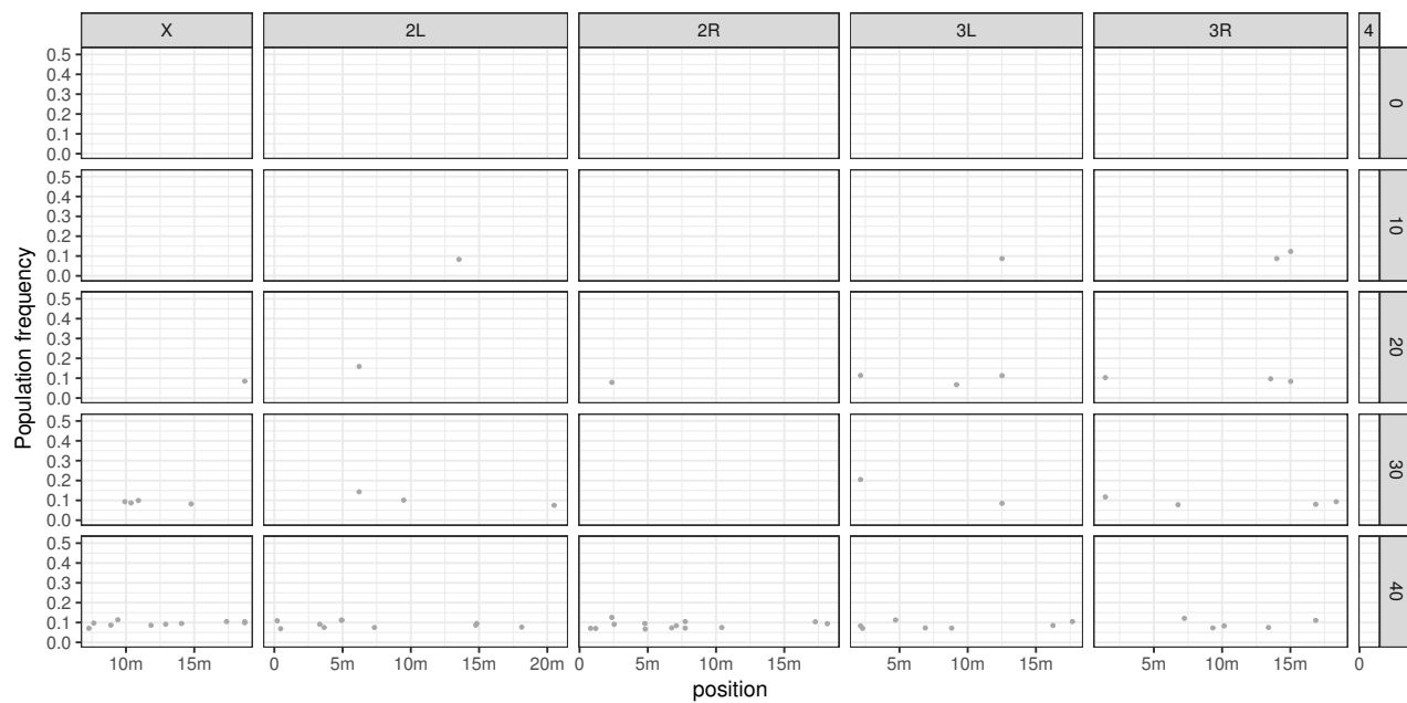
Supplementary Fig. 4: P-element invasion in cold replicate 1. For details see fig. 1.
