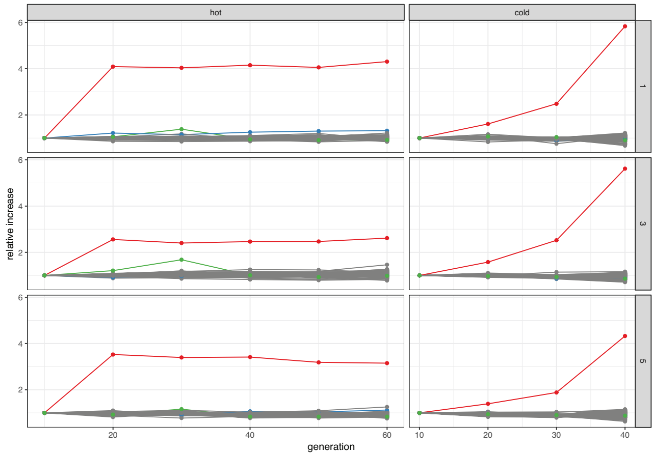
Supplementary Fig. 7: Abundance of 121 TE families (23 TIR, 60 LTR, 37 non-LTR and 1 Foldback) during the hot and cold invasion. Graphs show the fold-increase in reads mapping to each TE family relative to generation 10 (the base population consists solely of females whereas the evolved populations are a mix of males and females, which precludes a comparison of these two datasets). Results are shown for all three replicates (right panel) and two temperature regimes (top panel). Only the P-element (red) shows a pronounced increase in copy numbers; blue: mariner, green: BS
