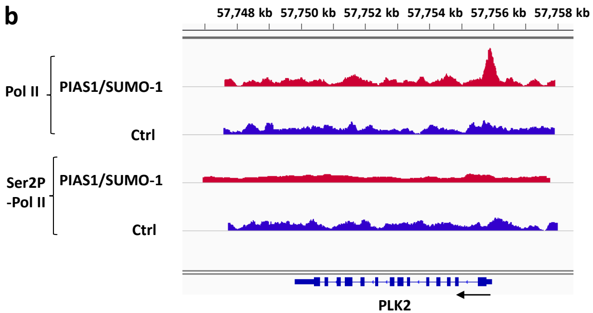
Supplementary Figure 10. UCSC genome browser views of Pol II and Ser2P ChIP-seq data at EIF2S3 ( a ) and PLK2 ( b ) gene loci. Arrow indicates the direction of transcription. Note significantly increased paused Pol II at the 5' ends for both genes.
