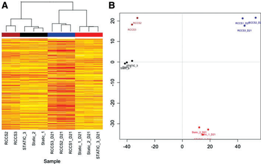
SUPPLEMENTARY FIG. S1. Microarray analysis in an iPSC Kit-Cre model of microgravity-induced cardiomyopathy. (A) Hierarchical clustering of 11 samples on 41345 genes that differentially express among groups. (B) Principal component analysis of 11 samples on 41345 genes, samples belonging to a group cluster together and four groups are well separated from each other. iPSC, induced pluripotent stem cells.
