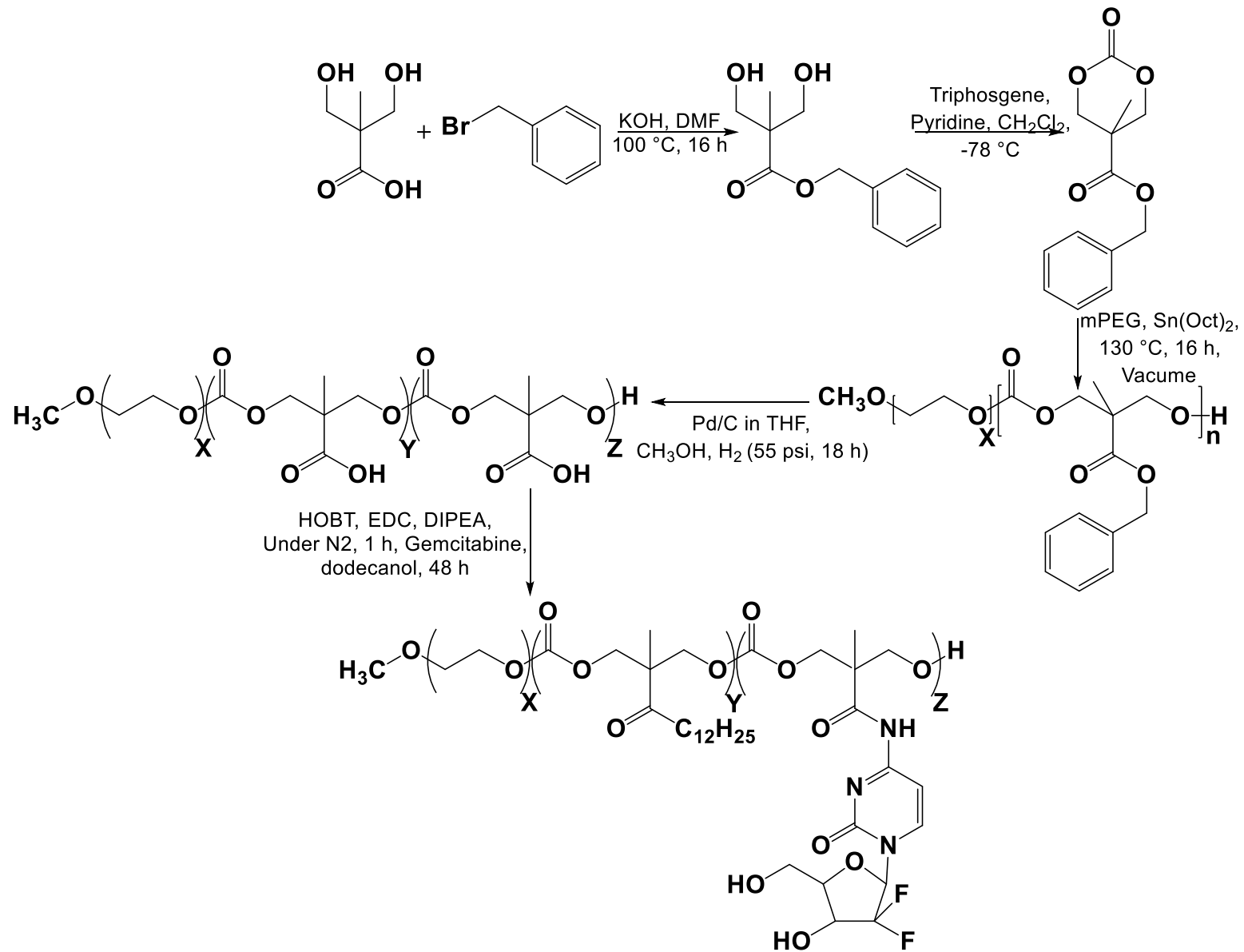
Figure S1. Synthesis scheme of mPEG-b-PCC-g-GEM-g-DC
