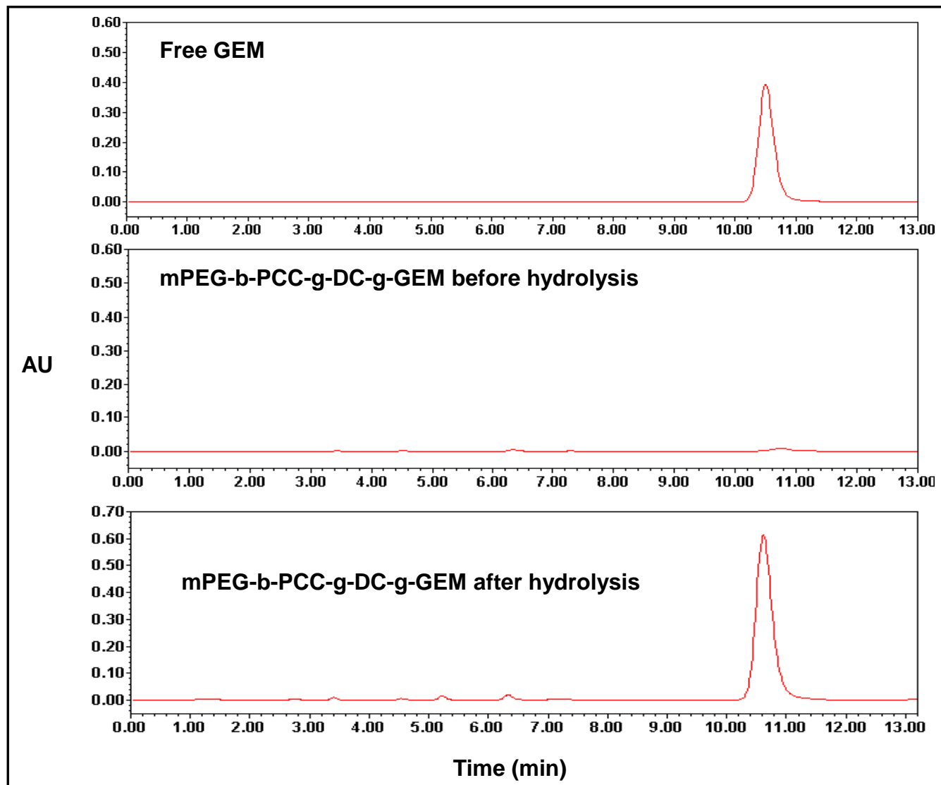
Figure S4. Gemcitabine payload in the formulation analyzed by HPLC, showing free Gemcitabine, polymer-Gemcitabine conjugate before and after hydrolysis.
