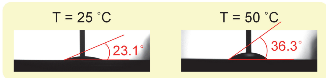
Supplementary Figure 1. Water contact angle on IPN gel below and above its LCST. The contact angles of water on the PNIPAAm/Alg IPN gel were measured at 25 °C (below LCST) and 50 °C (above LCST).
