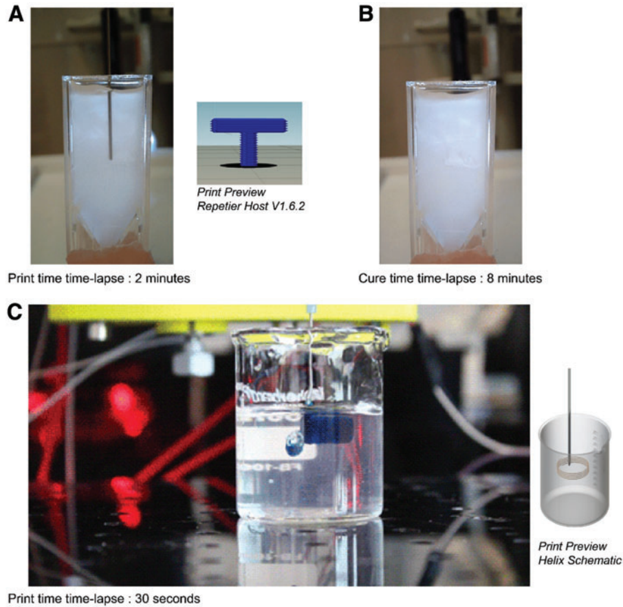
SUPPLEMENTARY FIG. S1. Schematic depicting phases of silk fibroin printing/curing and demonstration of freeform printing with dye with video legends. (A) Preview of Supplementary Video S1 with silk printing time lapse in curing medium. Print preview of T-shaped cantilever showing print paths generated in Repetier Host V1.6.2 shown in inset on right . (B) Preview of Supplementary Video S2 depicting curing of freeform-printed silk fibroin in time lapse over 8 min. (C) Preview of Supplementary Video S3 demonstrating freeform printing technique with helix printed with blue No. 2 dyed silk solution. Print preview schematic showing helical print path shown in inset on right . All syringe tips in videos 20G.
