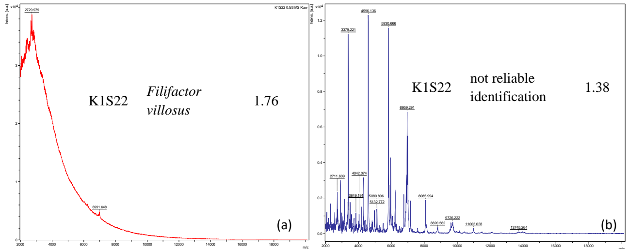
Fig. S2 MALDI-TOF MS spectra of isolate K1S22 indicating the differences in the spectral quality, MALDI biotyper database search for first spectrum (a) resulted genus level identity, whereas not reliable identification was obtained for second spectrum (b), the isolate was identified as Exiguobacterium acetylicum by 16S rRNA gene sequencing.
