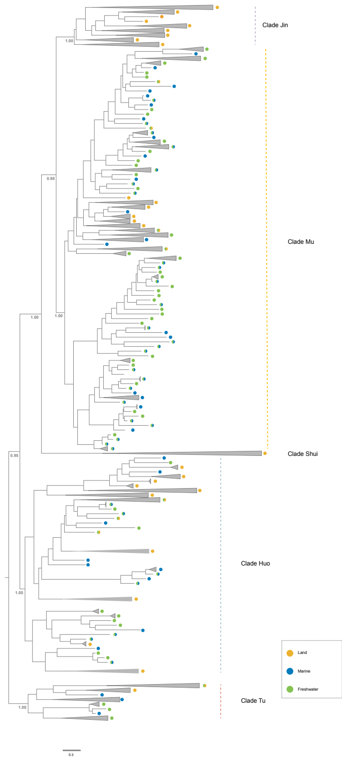
S3 Fig. Evolution of retroviruses at the land-water interface. The phylogenetic tree is based on Figure 1. The tip labels are based on the living environments of hosts.
