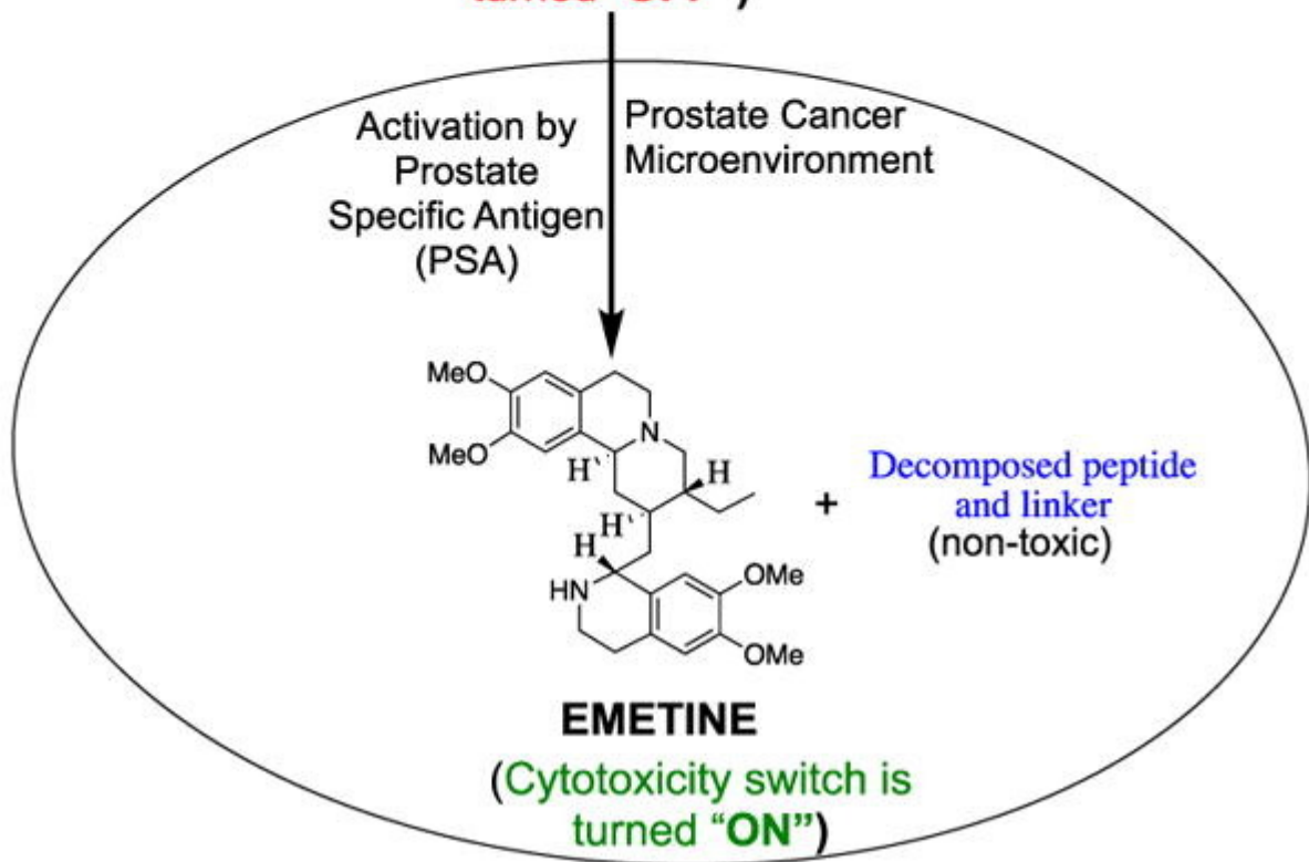
Emetine Prodrug (Cytotoxicity switch is turned "OFF")
