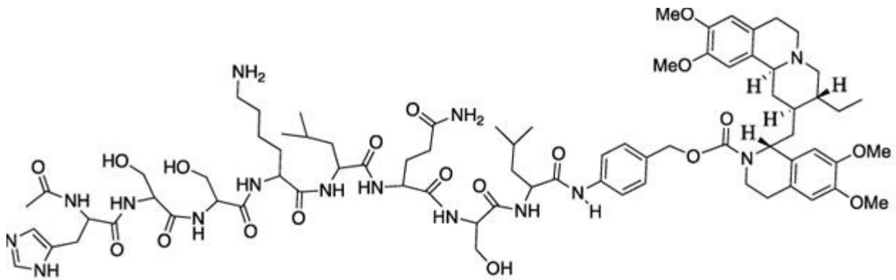
Emetine Prodrug (Cytotoxicity switch is turned "OFF")
