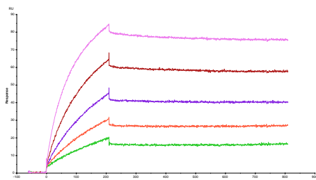
N49P7 gp120 (Chi 2 3.61; KD=8.602E-10)
