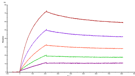
N49P11 gp120 (Chi 2 0.541; KD=1.562E-8)
