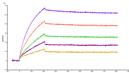
N49P9 gp120 (Chi 2 1.24; KD=2.456E-8)
