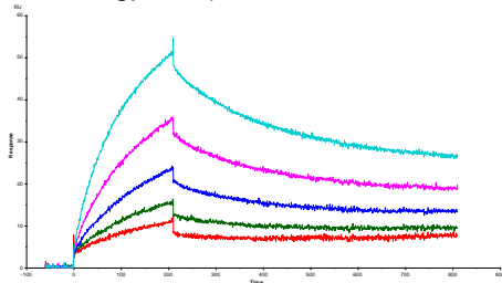
N49P6 gp120 (Chi 2 2.64; KD=1.59E-8)
