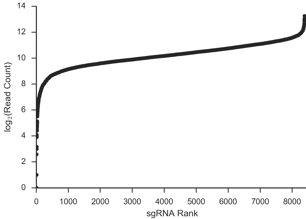
FIGURE S2. Read counts per sgRNA of the LX-miR plasmid library. The number of reads per sgRNA were plotted versus the rank of the sgRNA, from lowest to highest read count. Greater than 99% of the sgRNAs in the LX-miR library are represented in the plasmid pool with less than 5 fold difference in read counts between the 10 th and 90 th percentiles.
