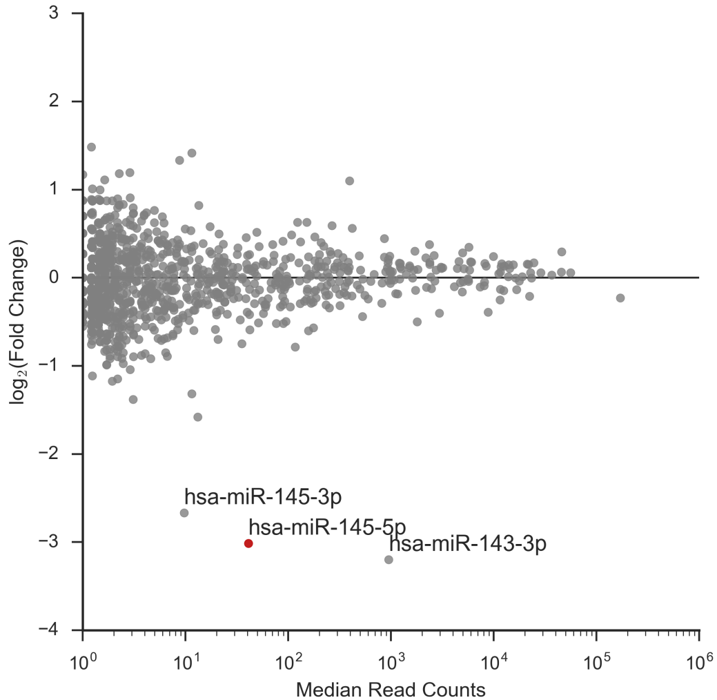
FIGURE S3. HeLa-Cas9 miRNA expression of initial and uninduced versus induced. The median read count is plotted versus the log2 fold change between the average of the initial and uninduced HeLa-Cas9 LX-miR pools and the induced HeLa-Cas9 LX-miR pool. The labeled miRNAs have a greater than 4 fold decrease after induction and the red dot indicates miR-145-5p, the only miRNA whose expression changed significantly after induction (DESeq2 adjusted p-value < 0.05).
