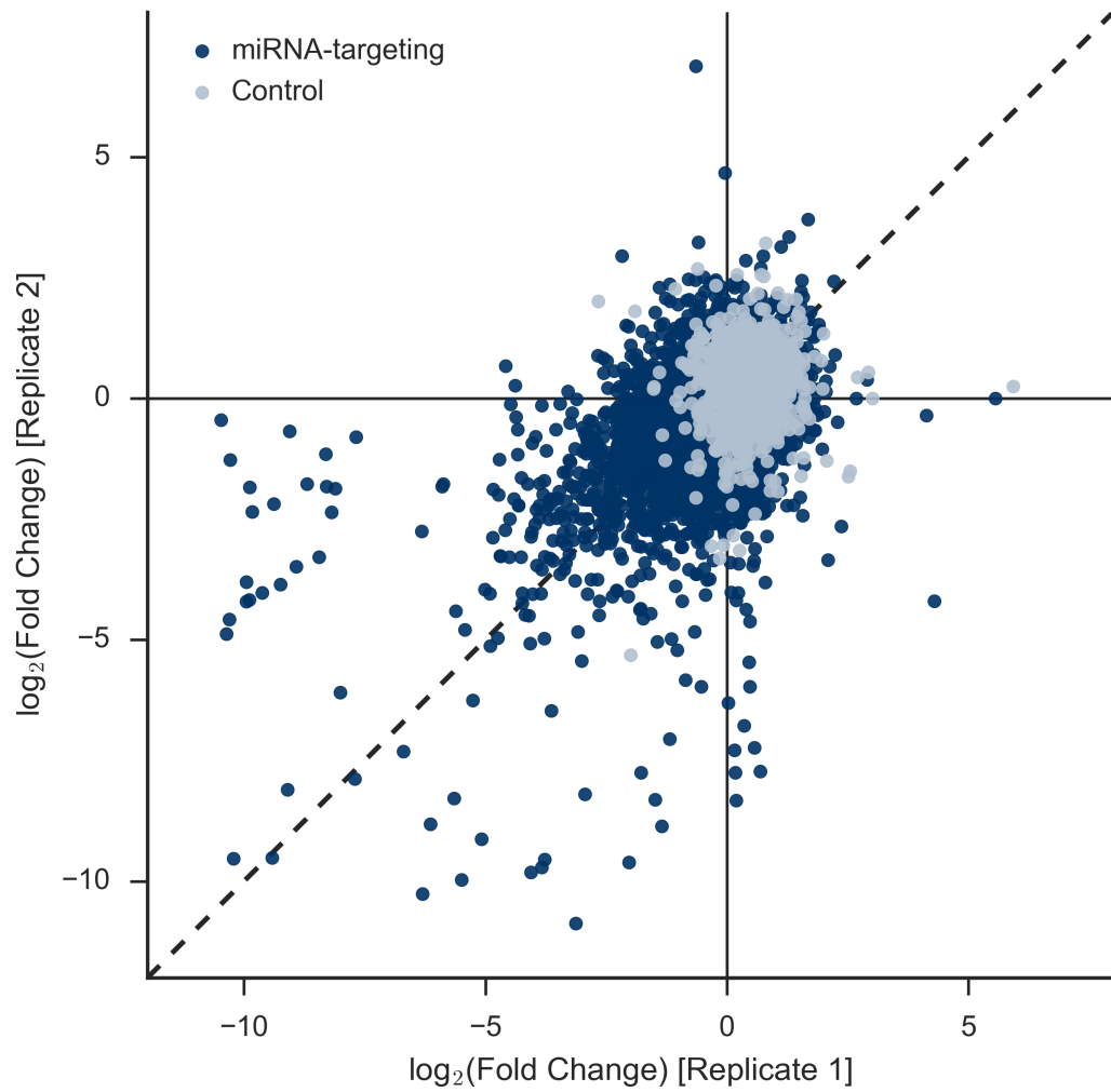
FIGURE S4. HeLa LX-miR Screen Fold Change Replicate 1 vs Replicate 2. The fold change for each sgRNA between replicates is significantly correlated (Pearson correlation coefficient: 0.46; p-value: 0.0).
