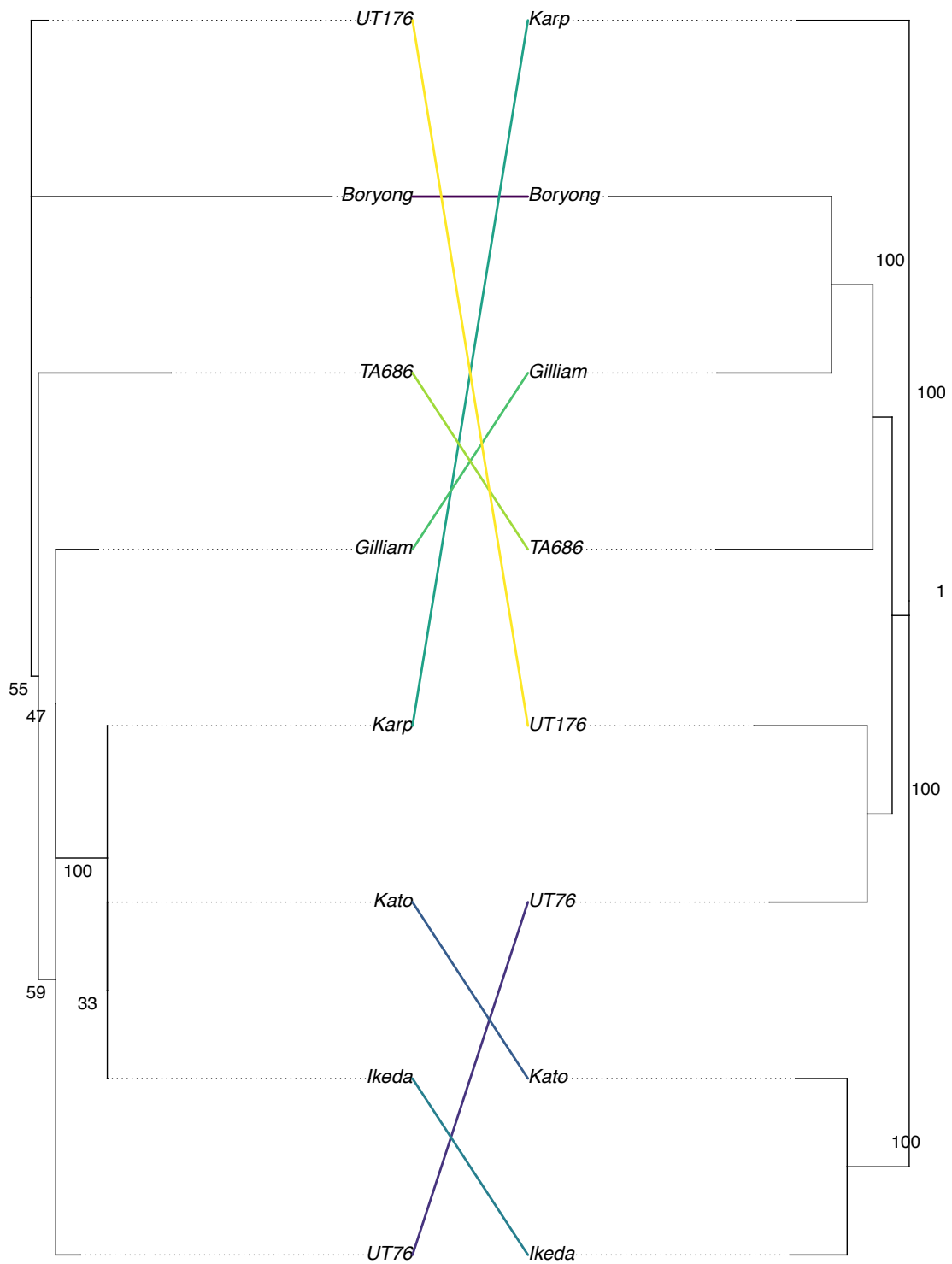
Figure S7. A phylogenetic tree showing the relationship between a tree generated using the 47kDa antigen sequences, and the sequences of 657 core genes.
