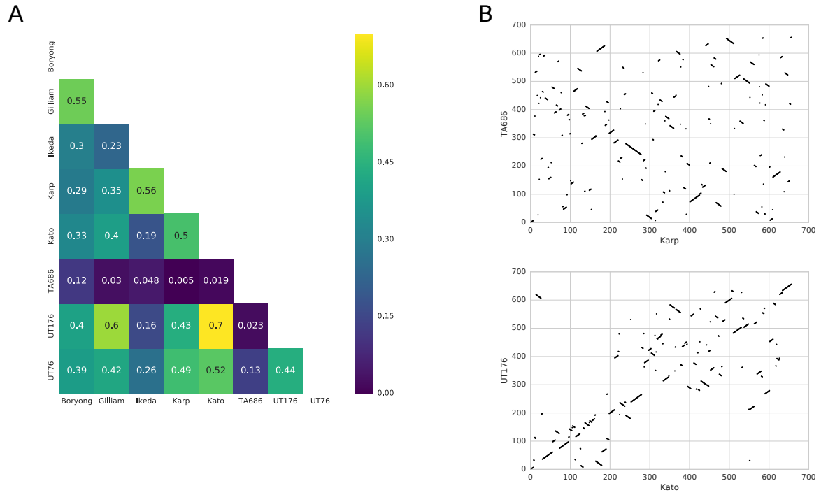
Figure S2. A - Heatmap showing the correlation in gene order between each pair of samples. B – dotplots showing the gene ordering between the pair with the highest correlation (Kato and UT176) and the lowest correlation (Karp and TA686).
