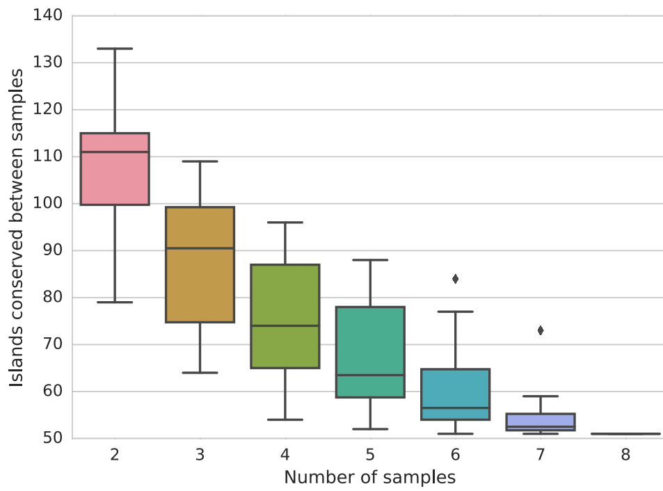
Figure S3. Boxplot showing the number of islands conserved between samples across all different combinations of samples.
