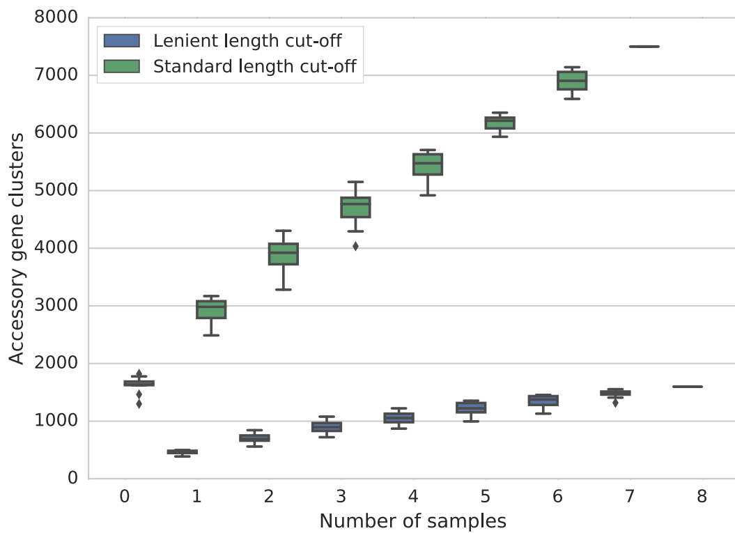
Figure S1. Boxplot showing how the number of accessory genes clusters varies with number of samples using the standard length cut-off and a more lenient length cut-off when determining clusters. Using the same identity thresholds but allowing the genes to be shorter reduces the number of new clusters identified as samples are added.
