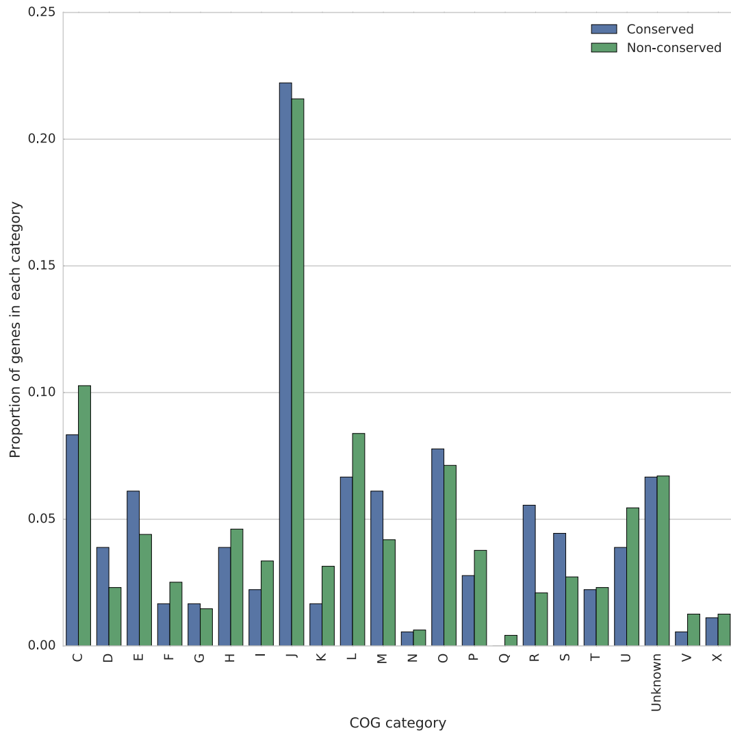
Figure S6. The proportion of core genes which are in conserved and non-conserved islands in each COG category.
