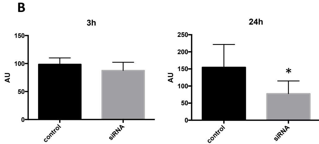
Figure S2: Quantification of G6PD protein expression following siRNA silencing approach. Protein quantification was assessed at 3 hours and 24 hours of neuronal differentiation, which corresponds to 27 hours and 48 hours of siRNA silencing, respectively. (A) Representative western blot membrane for each time point; (B) western blot band quantification. * p-value<0.05.
