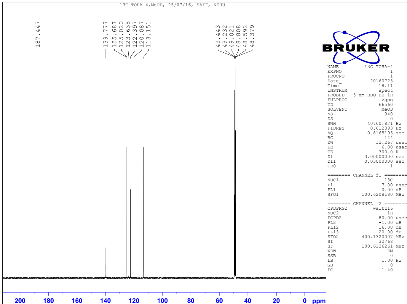
^{13}\text{C} NMR spectrum of compound 3''d
